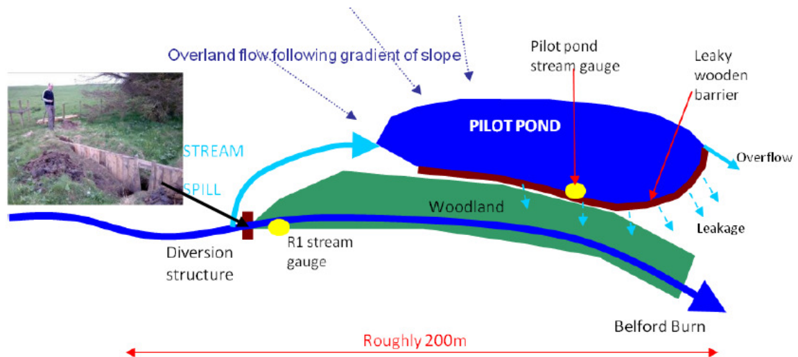
Figure 5 – Schematic of storage pond with a timber in-channel spill feature and leaky timber bund
