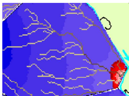
Figure 16 – Lidar being used to identify overland flow pathways and low points
